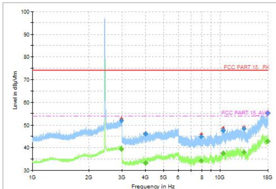
Fig.45 Radiated Spurious Emission (802.11n HT20, CH6, 1GHz-18GHz)
