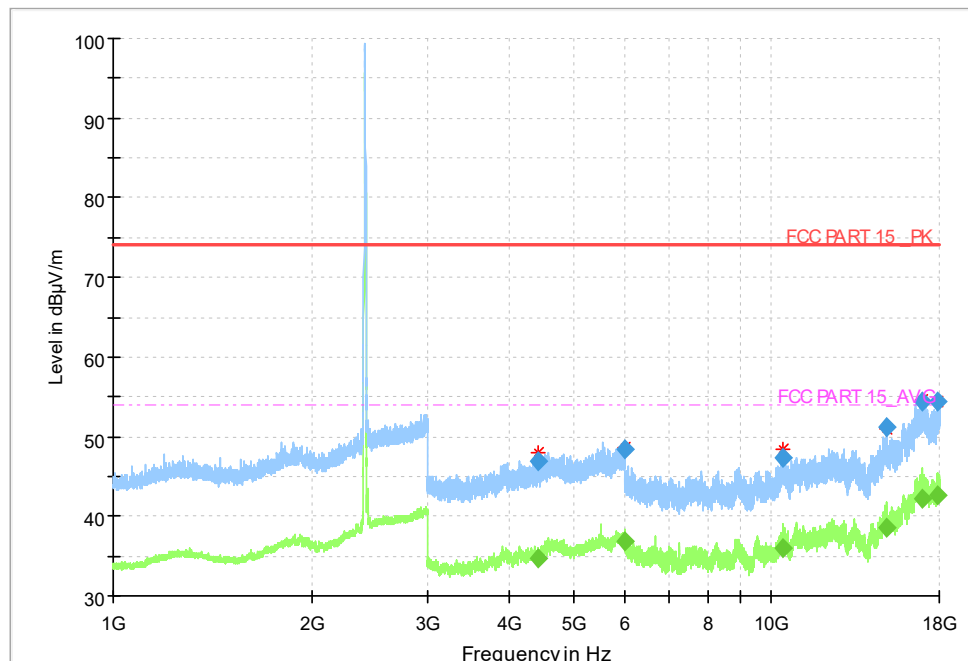
Fig.34 Radiated Spurious Emission (802.11b, CH1, 1GHz-18GHz)
