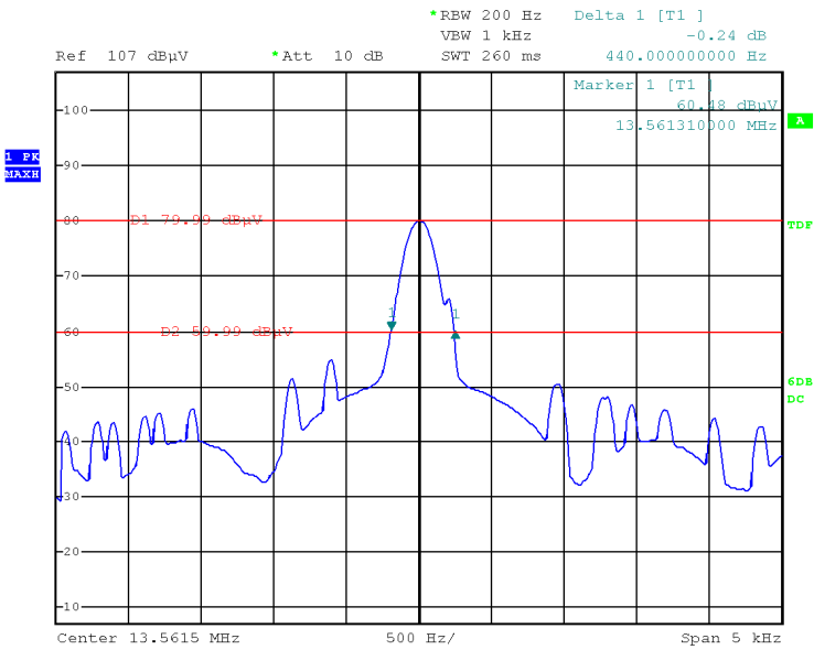
20 dB Emission Bandwidth-13.56MHz
