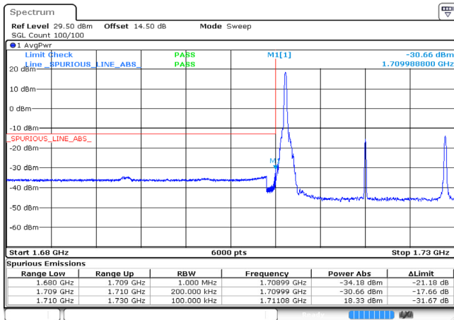
20MHz_Low_16QAM_1@0 -30.66dBm
