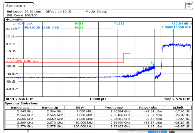
5MHz_Low_16QAM_25@0 -29.64dBm
