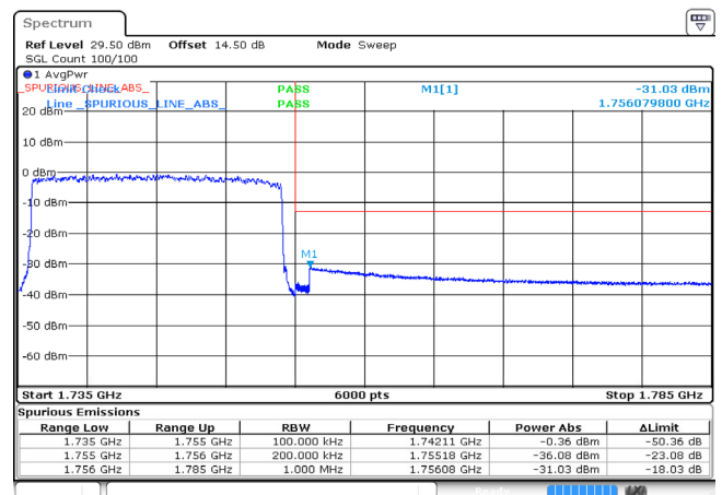
20MHz_High_16QAM_100@0 -31.03dBm
