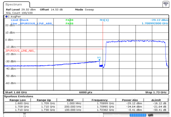
20MHz_Low_16QAM_100@0 -29.12dBm
