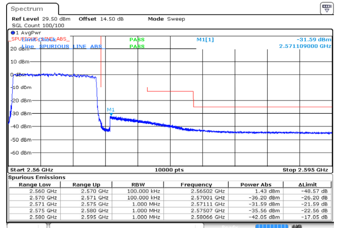
10MHz_High_16QAM_50@0 -31.59dBm
