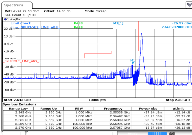
10MHz_Low_16QAM_1@0 -26.37dBm
