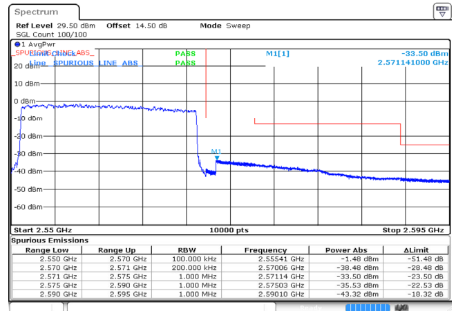
20MHz_High_16QAM_100@0 -33.50dBm
