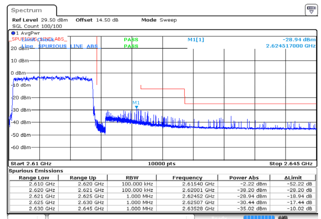
10MHz_High_16QAM_50@0 -28.94dBm
