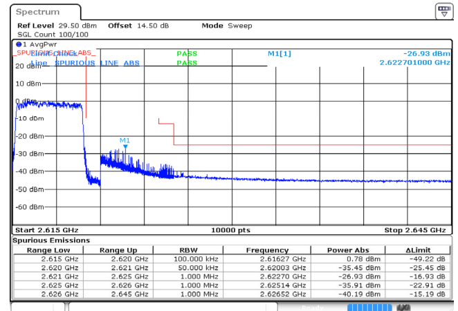
5MHz_High_16QAM_25@0 -26.93dBm
