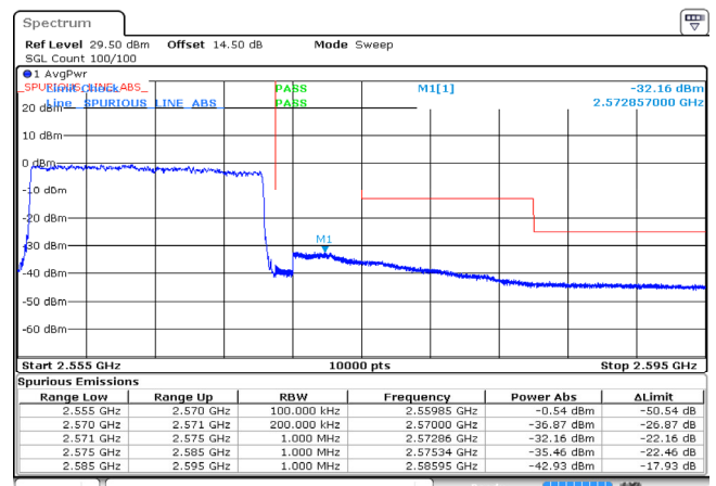
15MHz_High_16QAM_75@0 -32.16dBm
