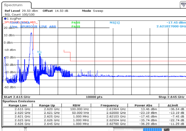
5MHz_High_16QAM_1@24 -17.45dBm
