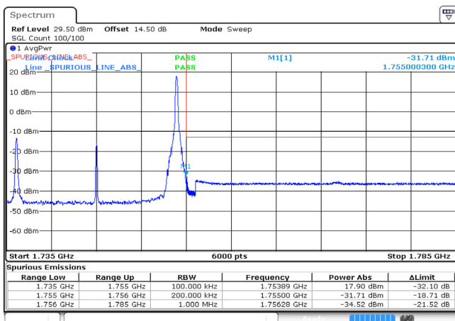
20MHz_High_16QAM_1@99 -31.71dBm
