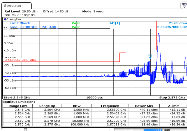
5MHz_Low_16QAM_1@0 -21.63dBm
