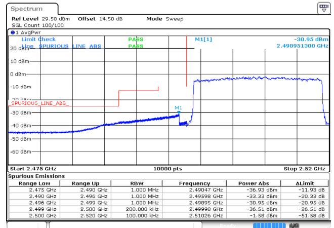
20MHz_Low_16QAM_100@0 -30.95dBm
