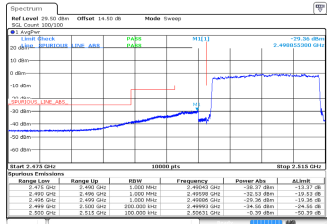
15MHz_Low_16QAM_75@0 -29.36dBm
