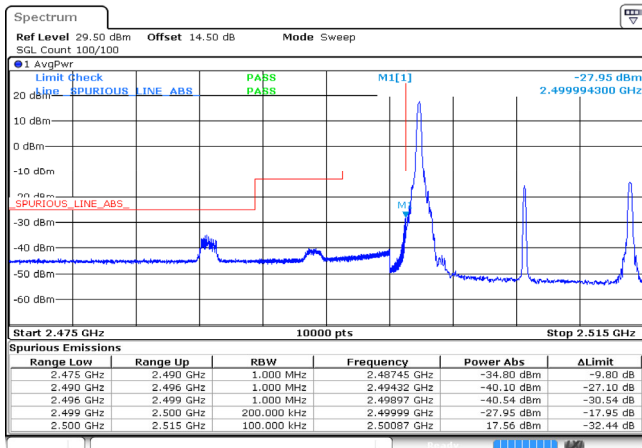
15MHz_Low_16QAM_1@0 -27.95dBm
