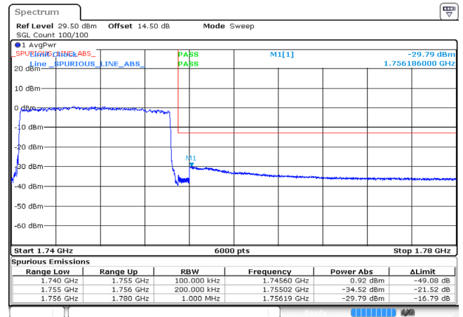
15MHz_High_16QAM_75@0 -29.79dBm
