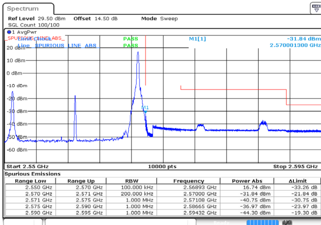
20MHz_High_16QAM_1@99 -31.84dBm
