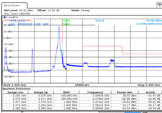
15MHz_High_16QAM_1@74 -26.80dBm
