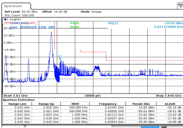
10MHz_High_16QAM_1@49 -23.62dBm
