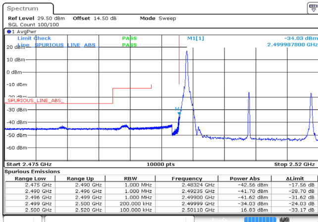
20MHz_Low_16QAM_1@0 -34.03dBm
