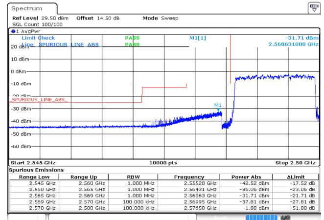
10MHz_Low_16QAM_50@0 -31.71dBm
