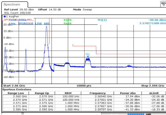
10MHz_High_16QAM_1@49 -30.06dBm
