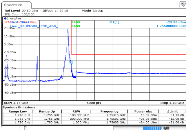
15MHz_High_16QAM_1@74 -25.98dBm
