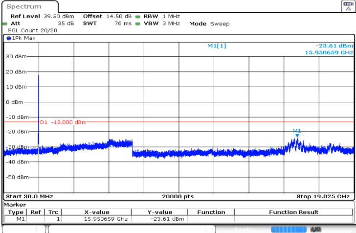
15MHz_High_QPSK_75@0 -23.61 dBm
