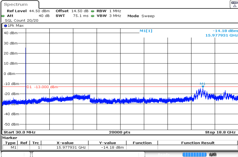
1.4MHz_Mid_QPSK_1@0 -14.18 dBm
