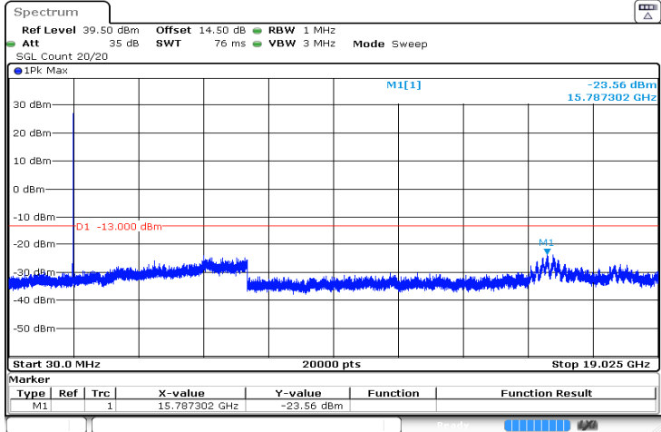
15MHz_High_QPSK_1@0 -23.56 dBm
