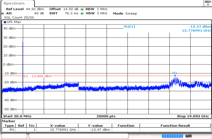
1.4MHz_High_QPSK_1@0 -13.47 dBm
