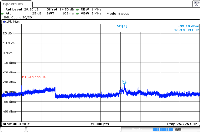
5MHz_Low_QPSK_25@0 -33.10 dBm
