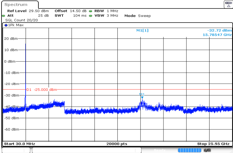
20MHz_Mid_QPSK_100@0 -32.72 dBm
