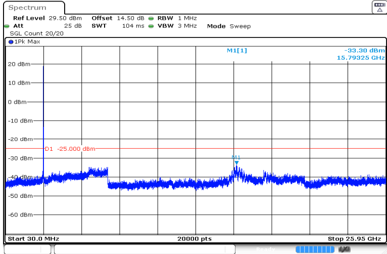
10MHz_Mid_QPSK_50@0 -33.30 dBm
