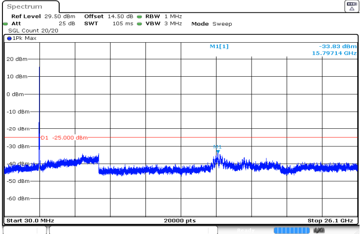
20MHz_High_QPSK_100@0 -33.83 dBm
