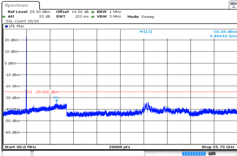
10MHz_Low_QPSK_1@0 -33.56 dBm
