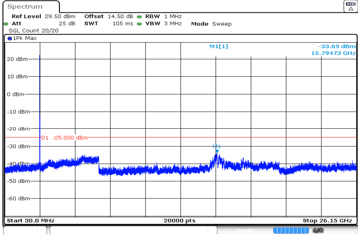
10MHz_High_QPSK_1@0 -33.69 dBm
