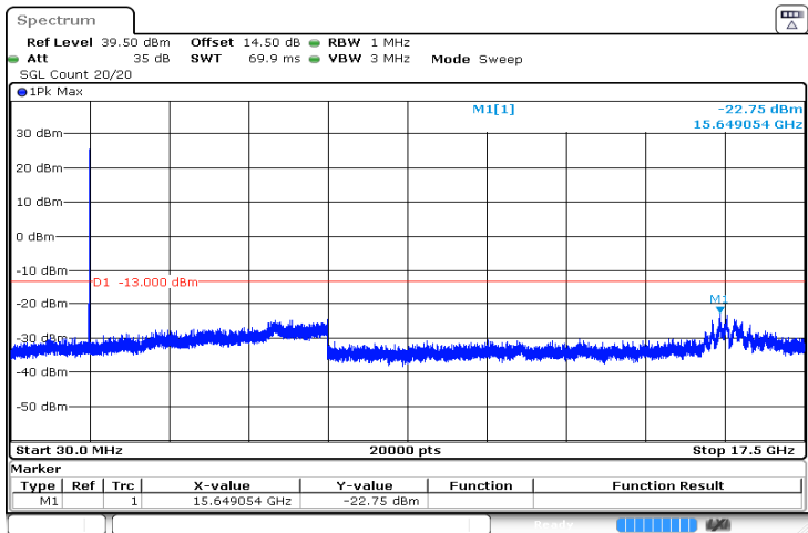
10MHz_High_QPSK_1@0 -22.75 dBm
