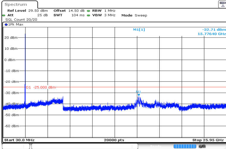
10MHz_Mid_QPSK_1@0 -32.71 dBm
