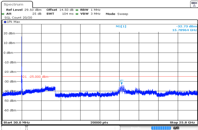
20MHz_Low_QPSK_100@0 -32.73 dBm
