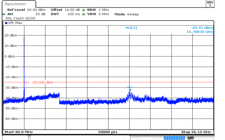
10MHz_High_QPSK_50@0 -33.41 dBm
