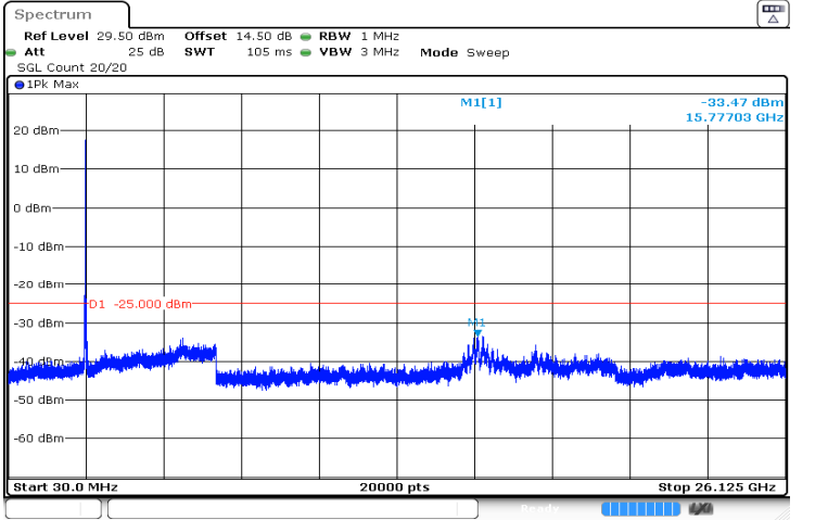
15MHz_High_QPSK_75@0 -33.47 dBm
