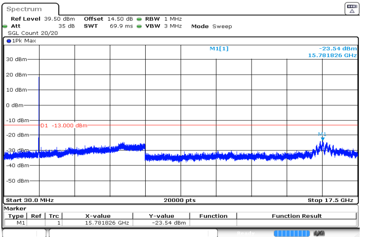
10MHz_High_QPSK_50@0 -23.54 dBm
