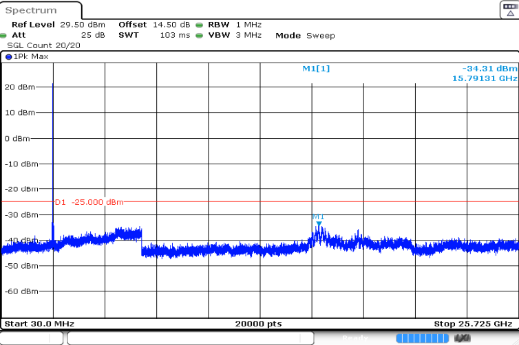
5MHz_Low_QPSK_1@0 -34.31 dBm
