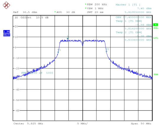
802.11a_5825MHz
