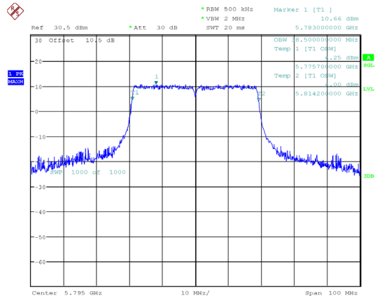
802.11ax40_5795MHz_RU_Full
