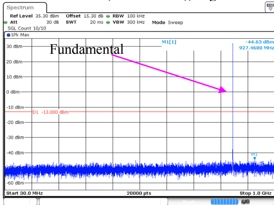
30 MHz – 1GHz (GPRS Mode), High channel
