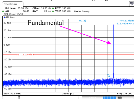
30 MHz – 1GHz (EGPRS Mode), High channel
