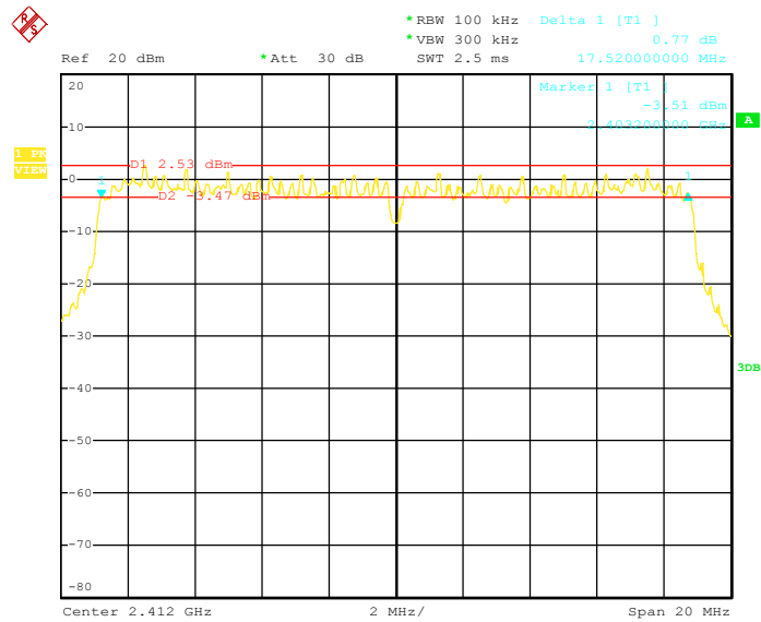
6dB Bandwidth (CH Low)
