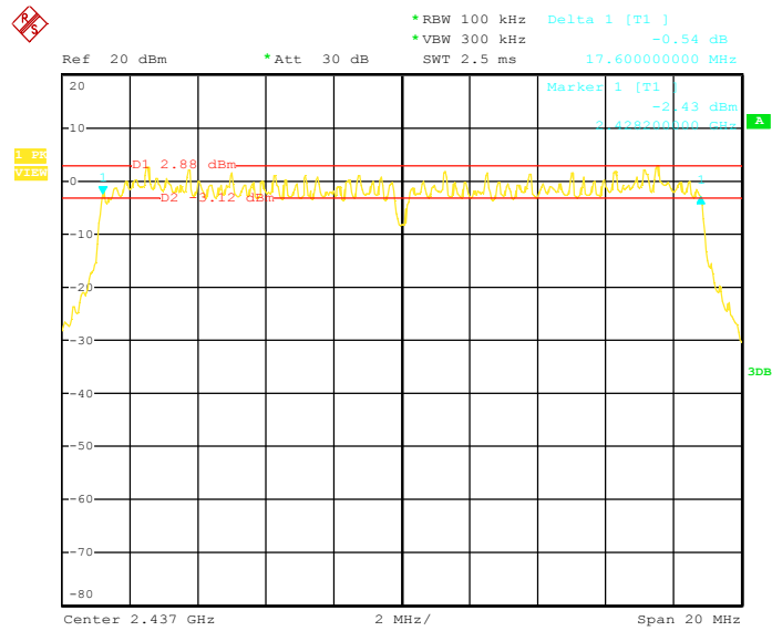
6dB Bandwidth (CH Mid)
