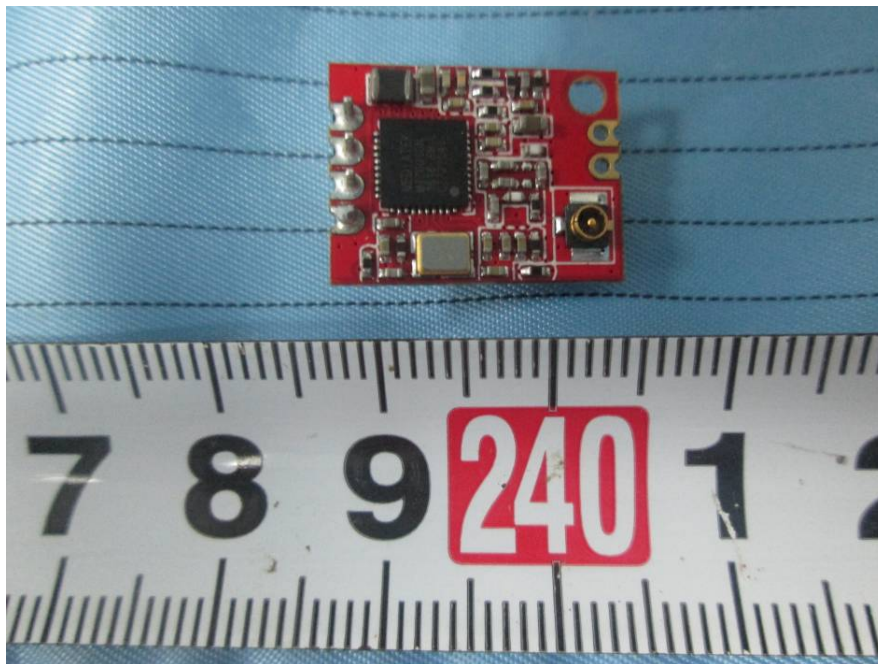
EUT –Wifi module Board Bottom View 1
