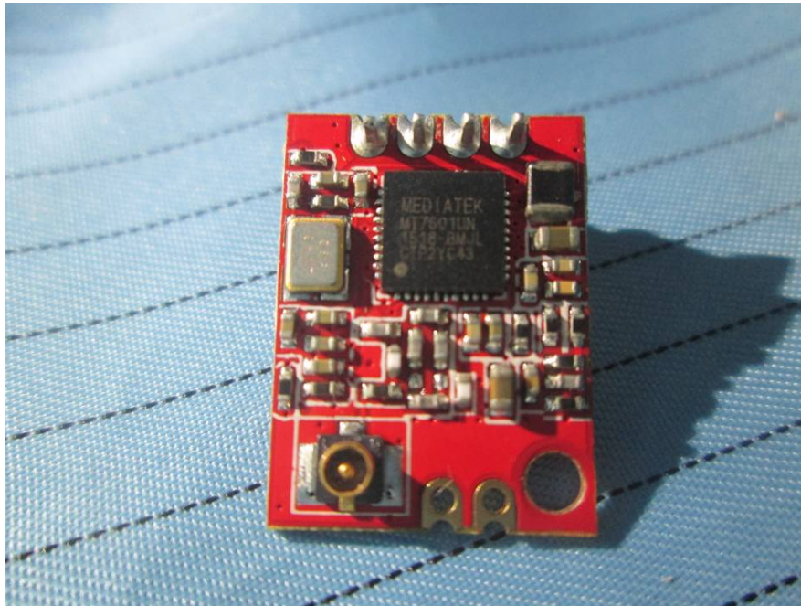
EUT –Wifi module Board bottom view 2
