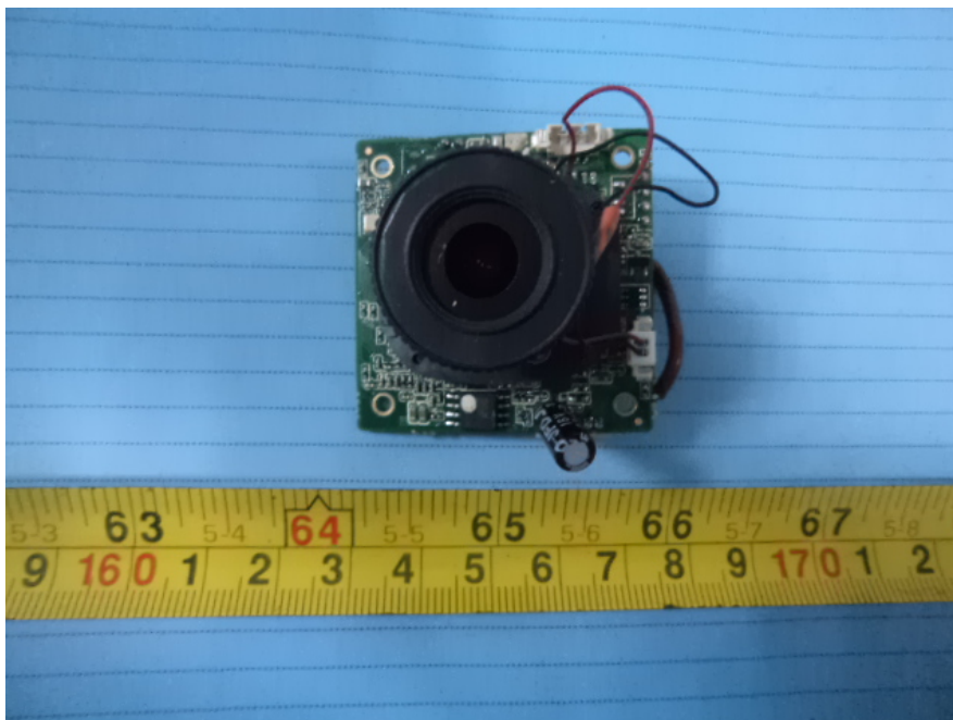
EUT – Main Board Top with Camera View
