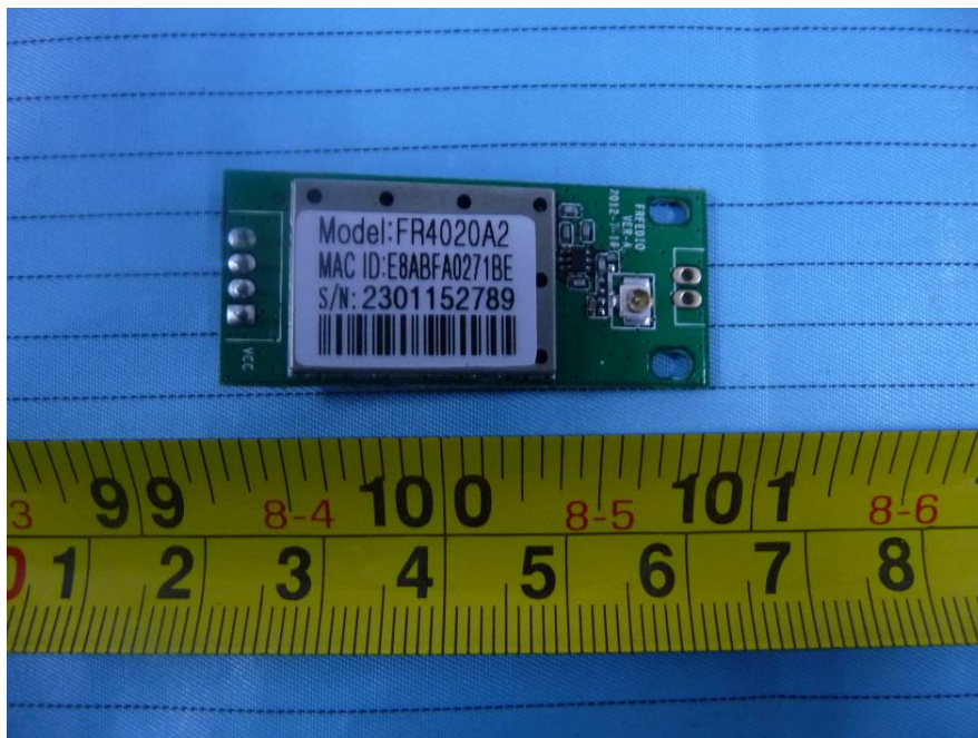
EUT – WiFi Module Board Top View
