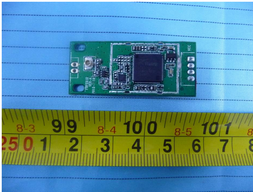
EUT – WiFi Module Board Top Shielding off View
