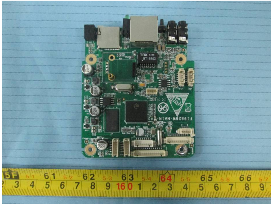
EUT – Main Board Front View 3
