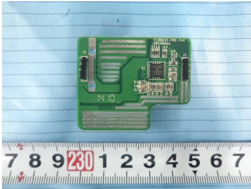
EUT –Module Bottom Shielding off View
