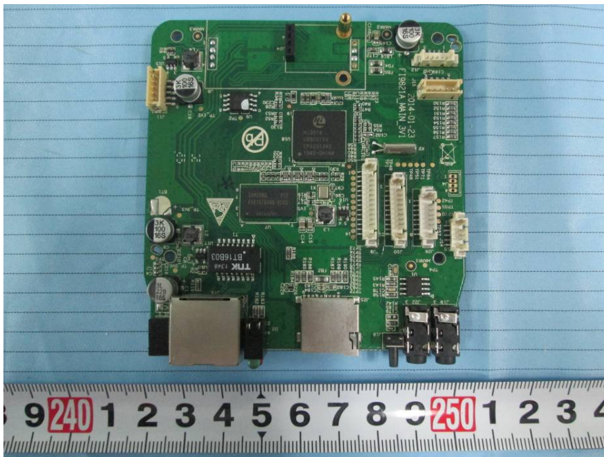
EUT – Main Board WIFI Module Off Top View
