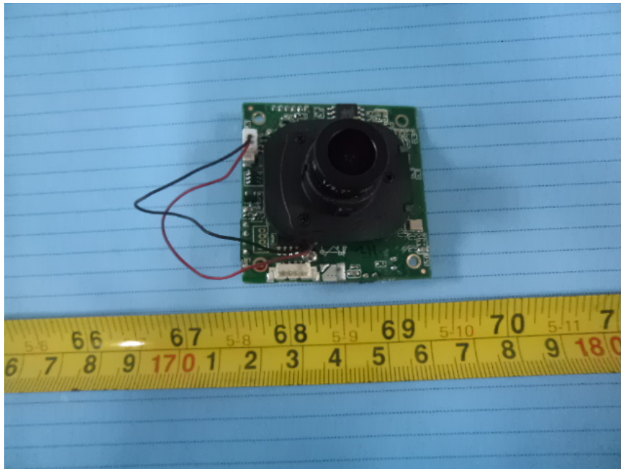
EUT – Main Board with Camera Top View
