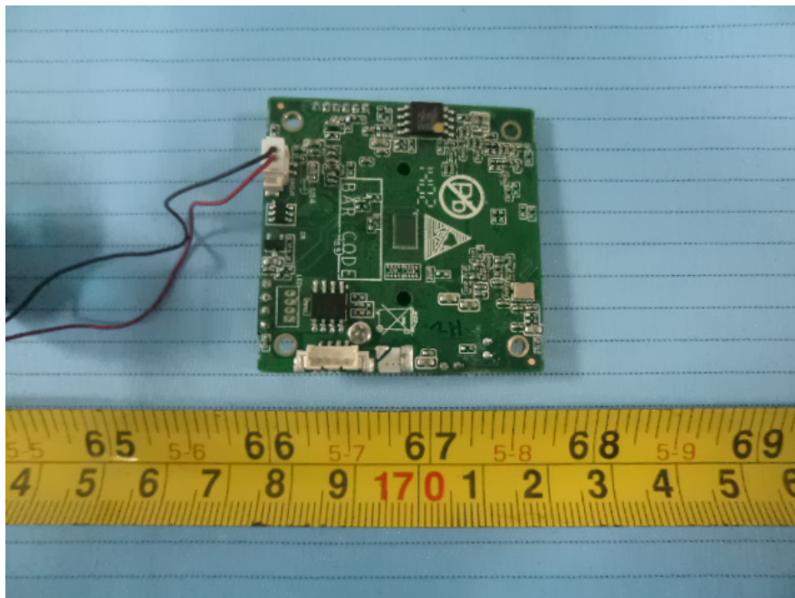
EUT – Main Board without Camera Top View
