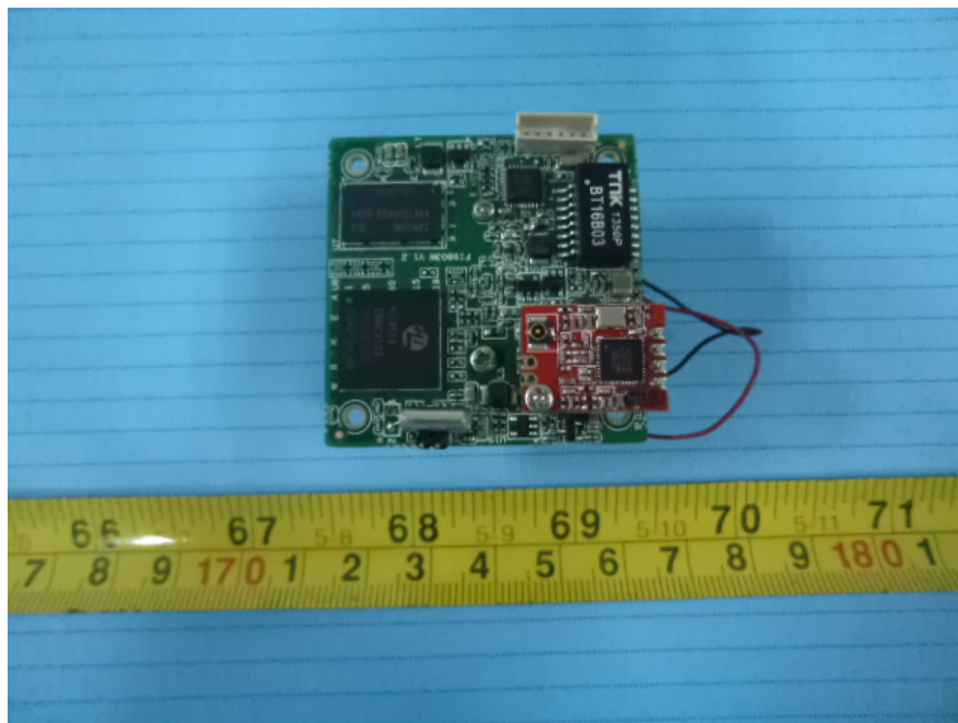
EUT – Main Board with WIFI Module View
