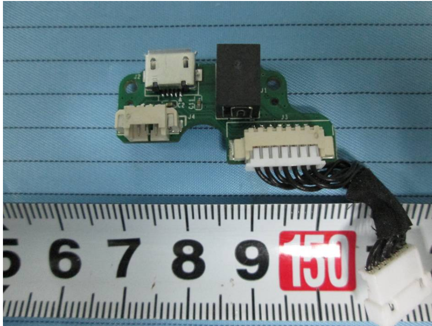
EUT – External Port PCB Top View
