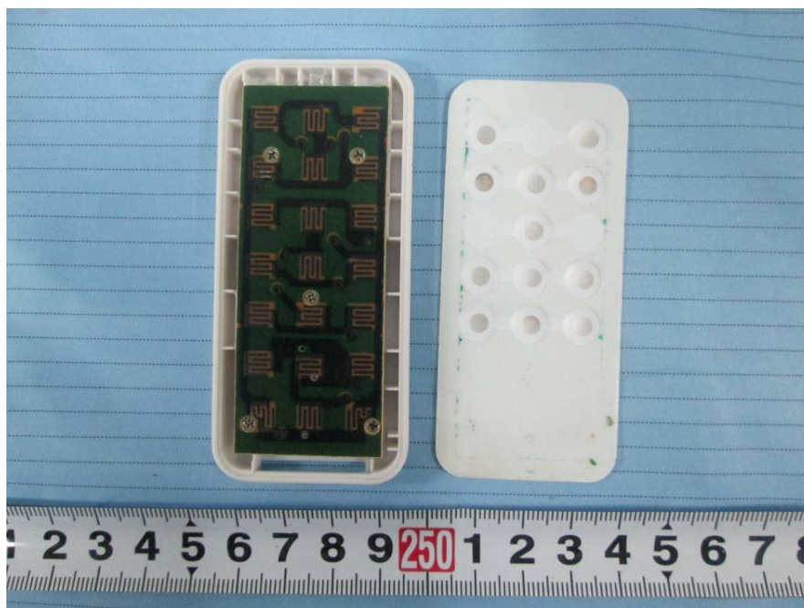
EUT – Cover off View 2 (Remote-controller)
