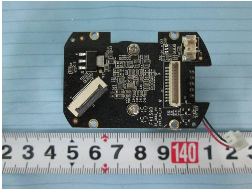
EUT – Image Sensor PCB Bottom View
