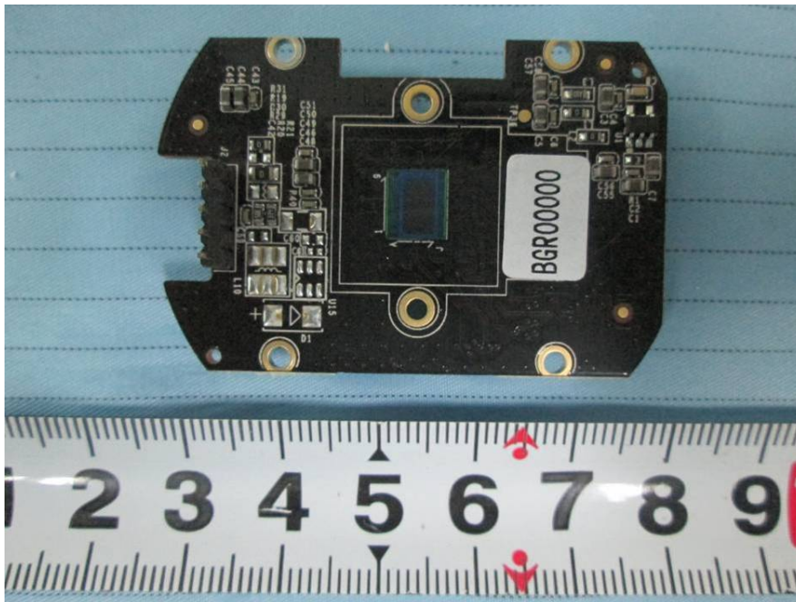
EUT – Image Sensor PCB Top Shielding Off View
