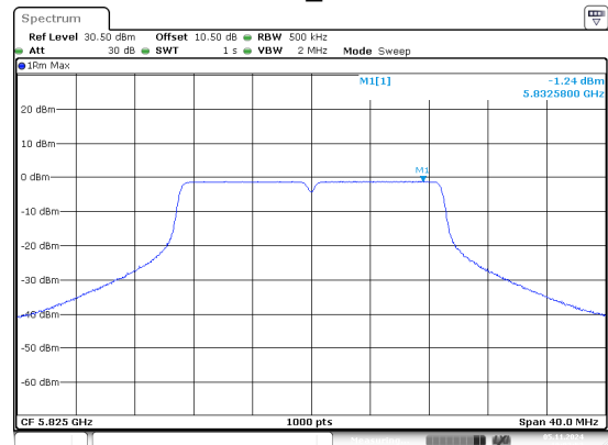
802.11n20_5825MHz
