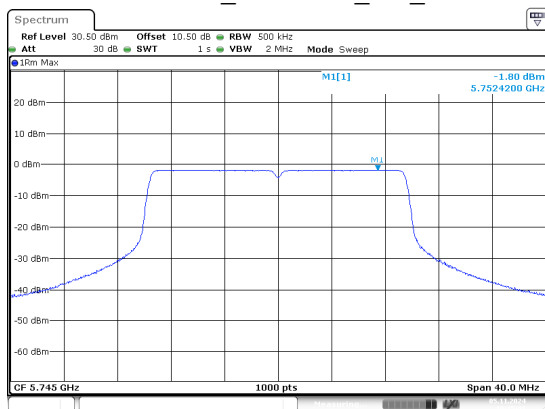
802.11ax20_5745MHz_RU_Full
