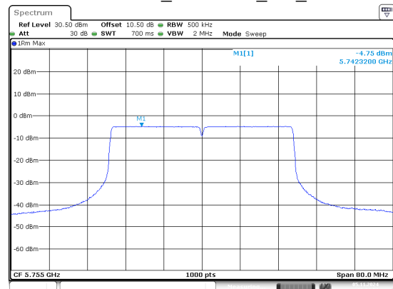
802.11ax40_5755MHz_RU_Full
