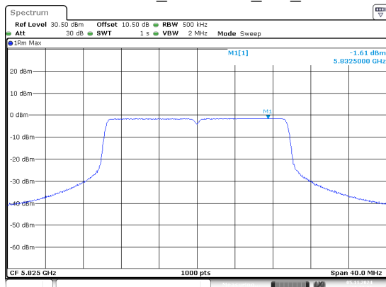
802.11ax20_5825MHz_RU_Full
