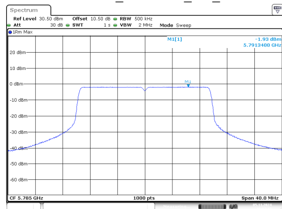
802.11ax20_5785MHz_RU_Full
