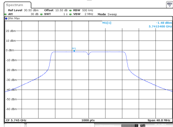
802.11n20_5745MHz
