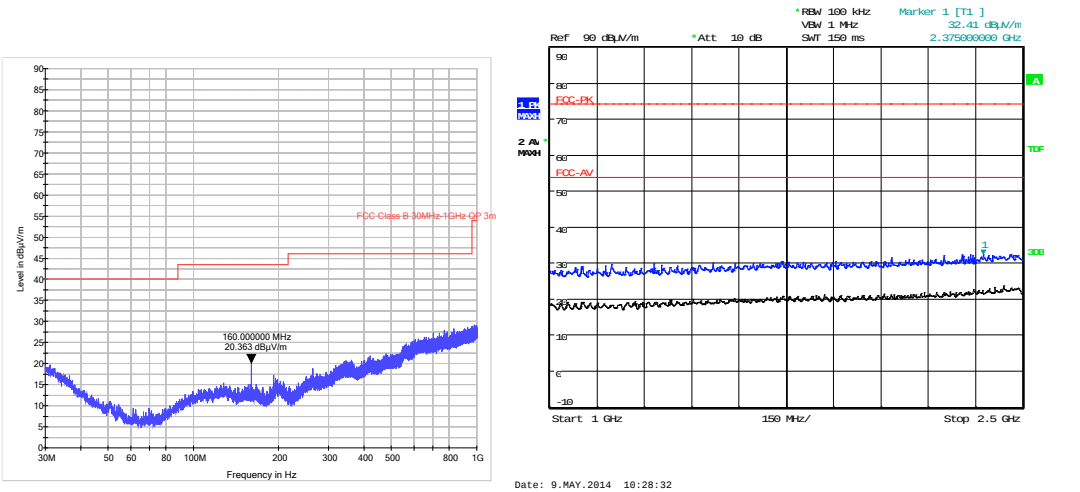
30MHz – 1GHz
