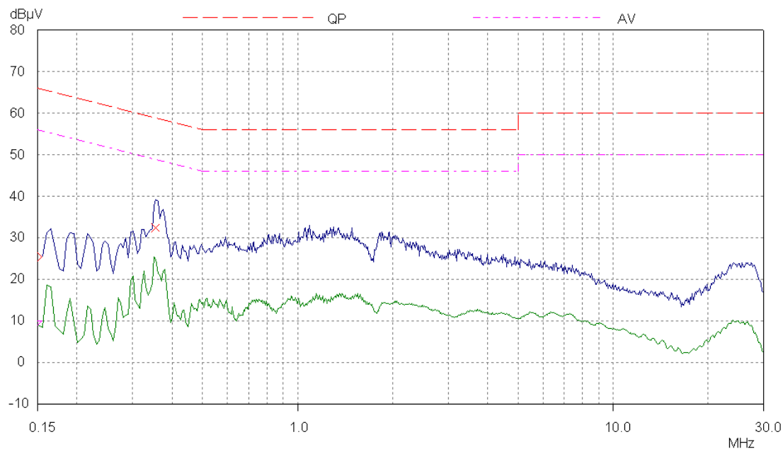
Neutral Line
