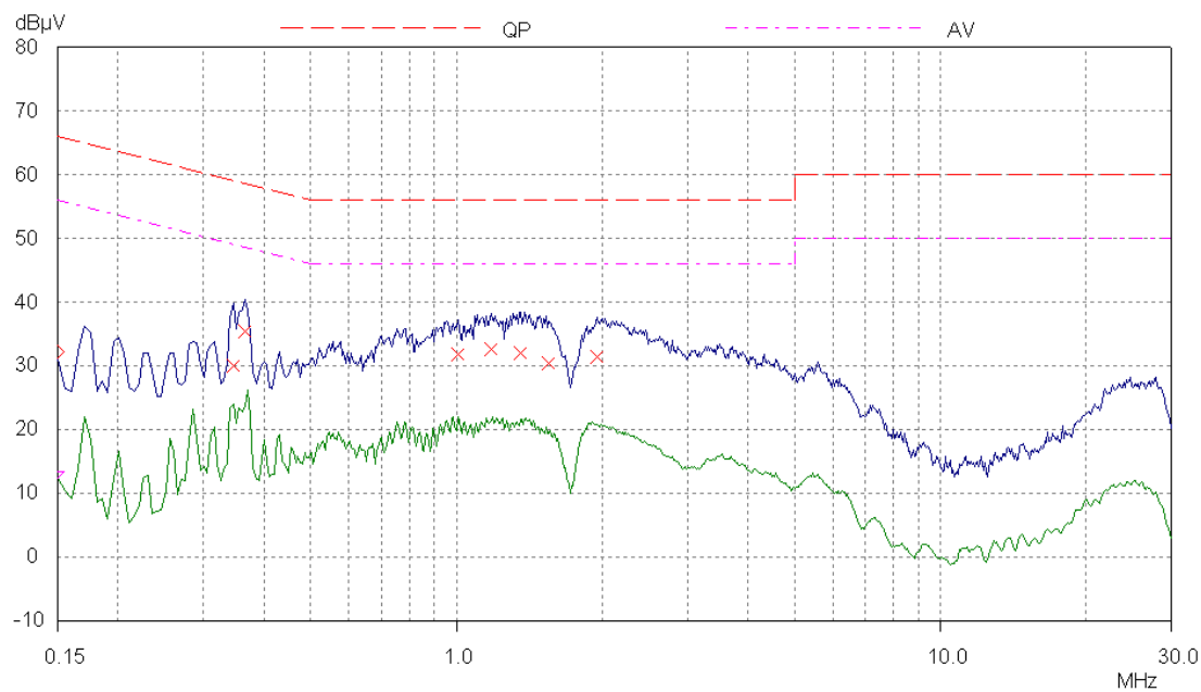
Live Line
