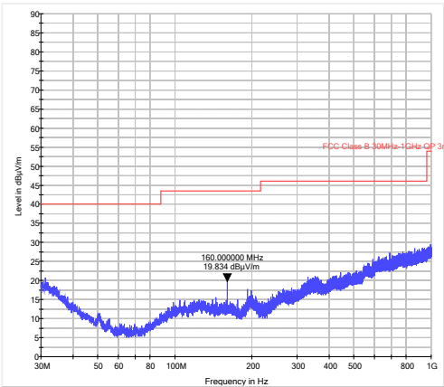
30MHz – 1GHz
