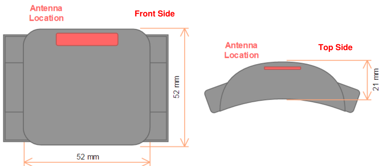
Fig. 1: Sketches of EUT and its antenna location (front and top side).
