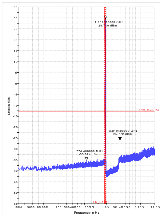
Diagram 36.31_RSE_Ch810_EGPRS_Sweep2
