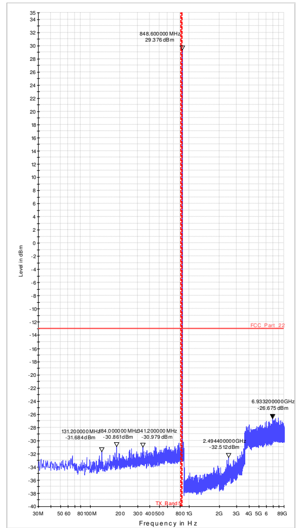
Diagram 36.18_RSE_Ch251_EGPRS_Sweep2
