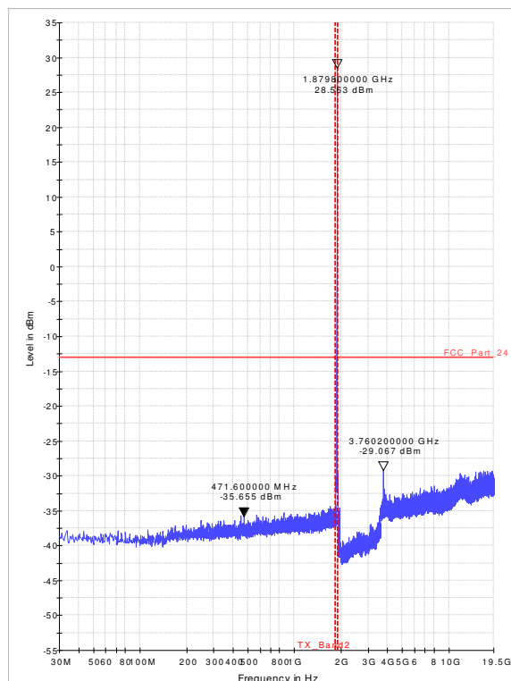
Diagram 36.29_RSE_Ch661_EGPRS_Sweep2
