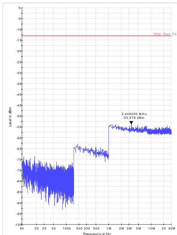
Diagram 36.28_RSE_Ch661_EGPRS_Sweep1
