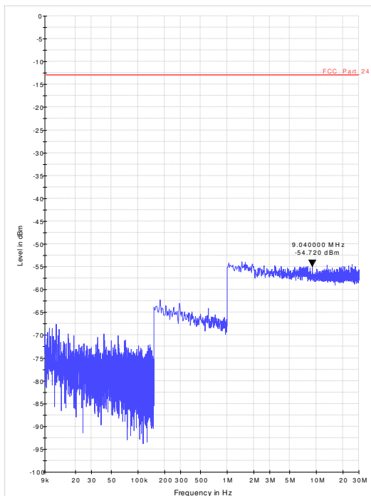
Diagram 36.30_RSE_Ch810_EGPRS_Sweep1
