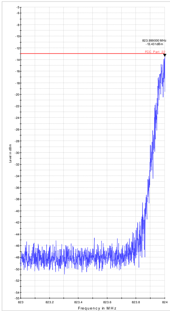
Diagram 37.03_BE_Ch128_GPRS
