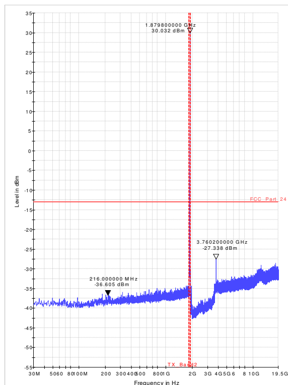
Diagram 36.23_RSE_Ch661_GPRS_Sweep2
