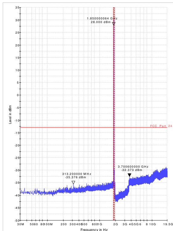
Diagram 36.21_RSE_Ch512_GPRS_Sweep2
