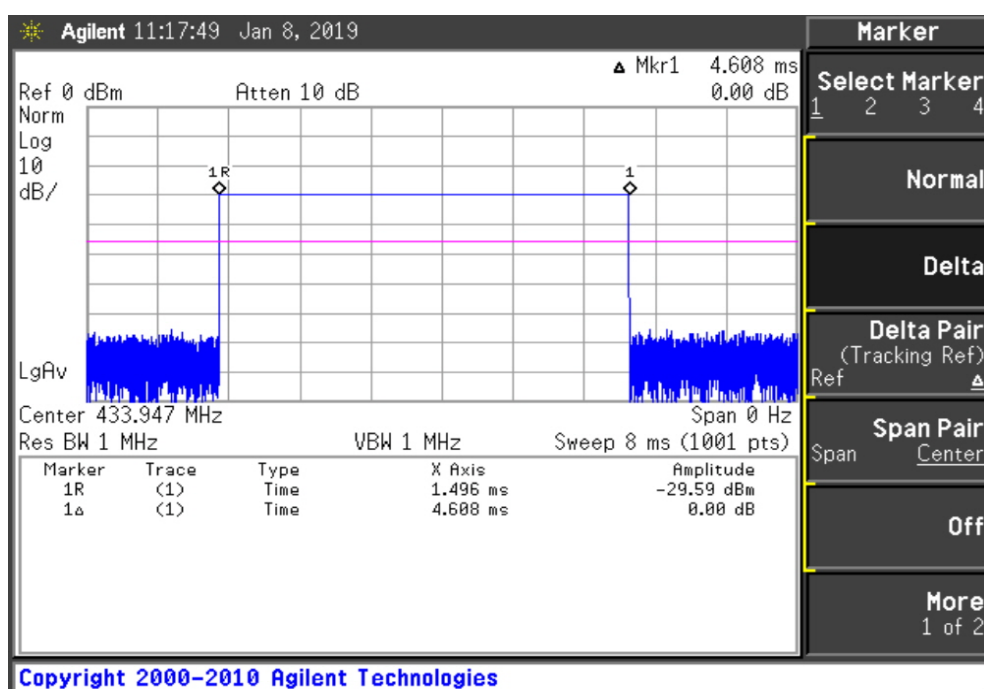
Duration of the burst signals
