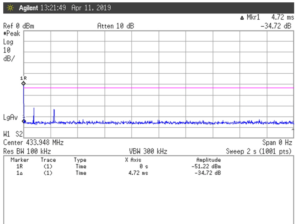
Figure 2. Plot of the Transmission Time (Operated from DC 12 V)
