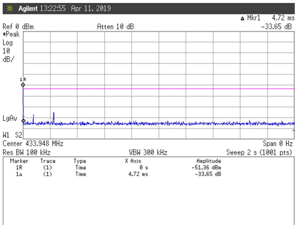
Figure 2. Plot of the Transmission Time (cont.) (Operated from DC 24 V)
