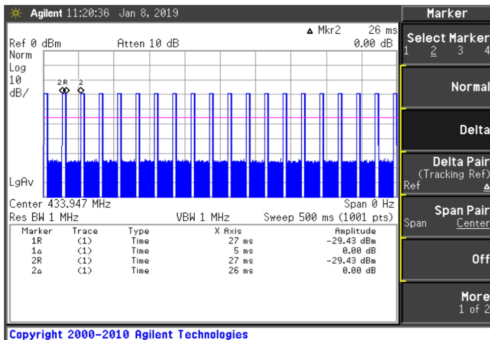
Periodic operation for the radiated emission measurements
