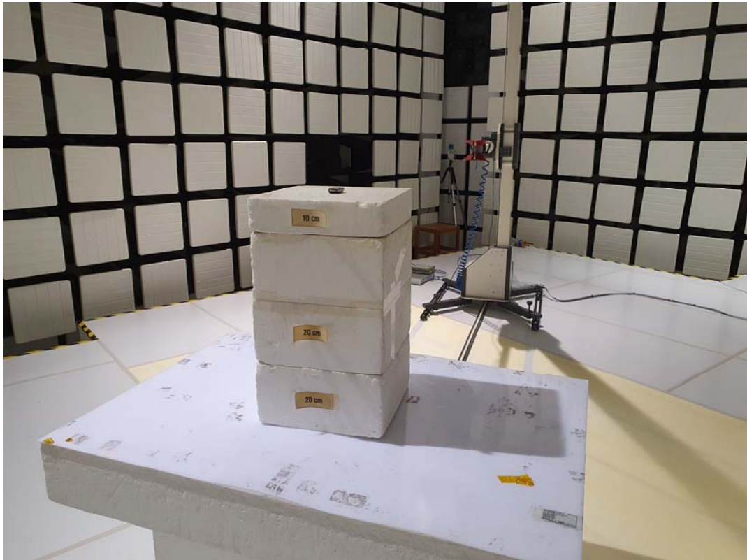
Radiated emission test (1 GHz to 5 GHz)
