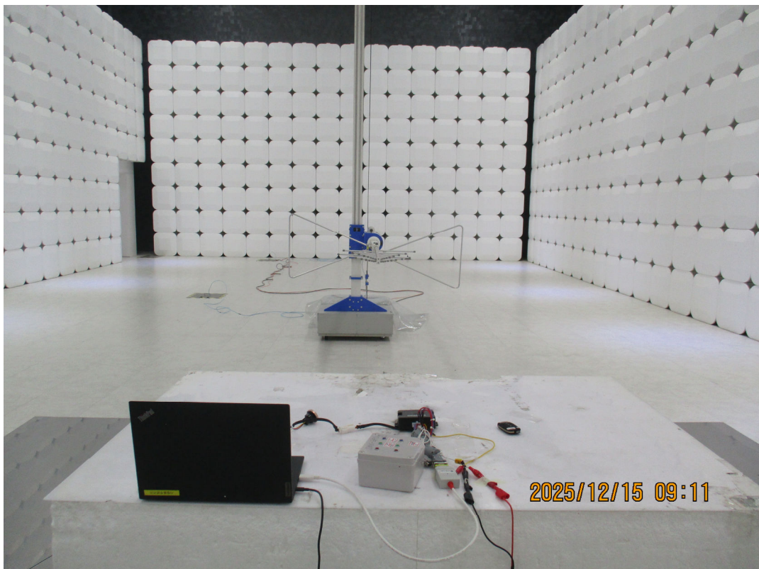
Radiated emission test (30 MHz to 1 GHz)
