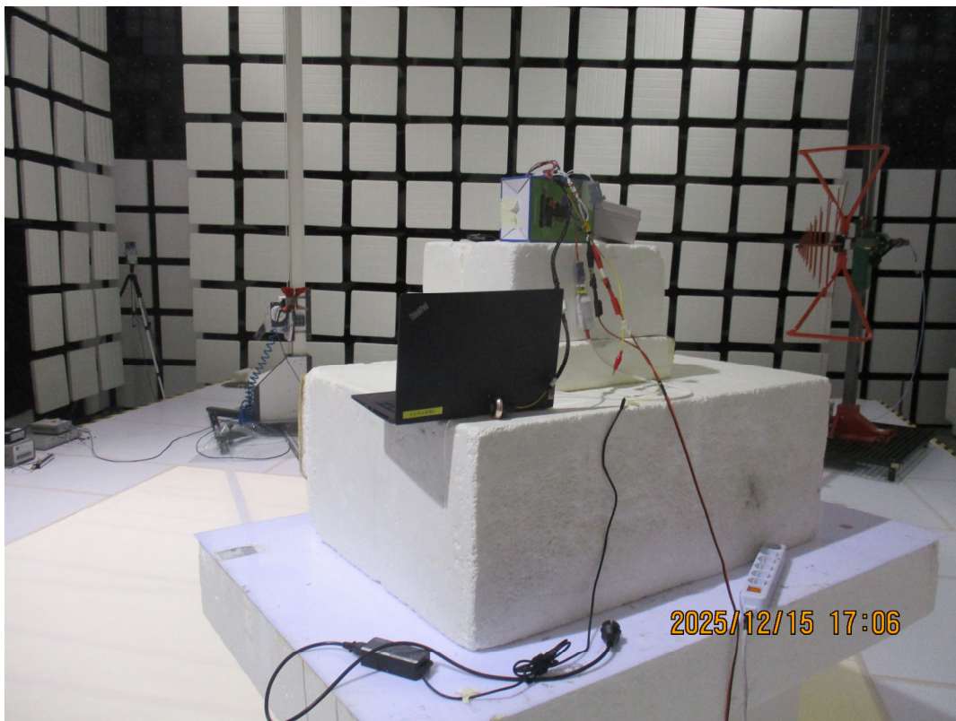
Radiated emission test (1 GHz to 6 GHz)
