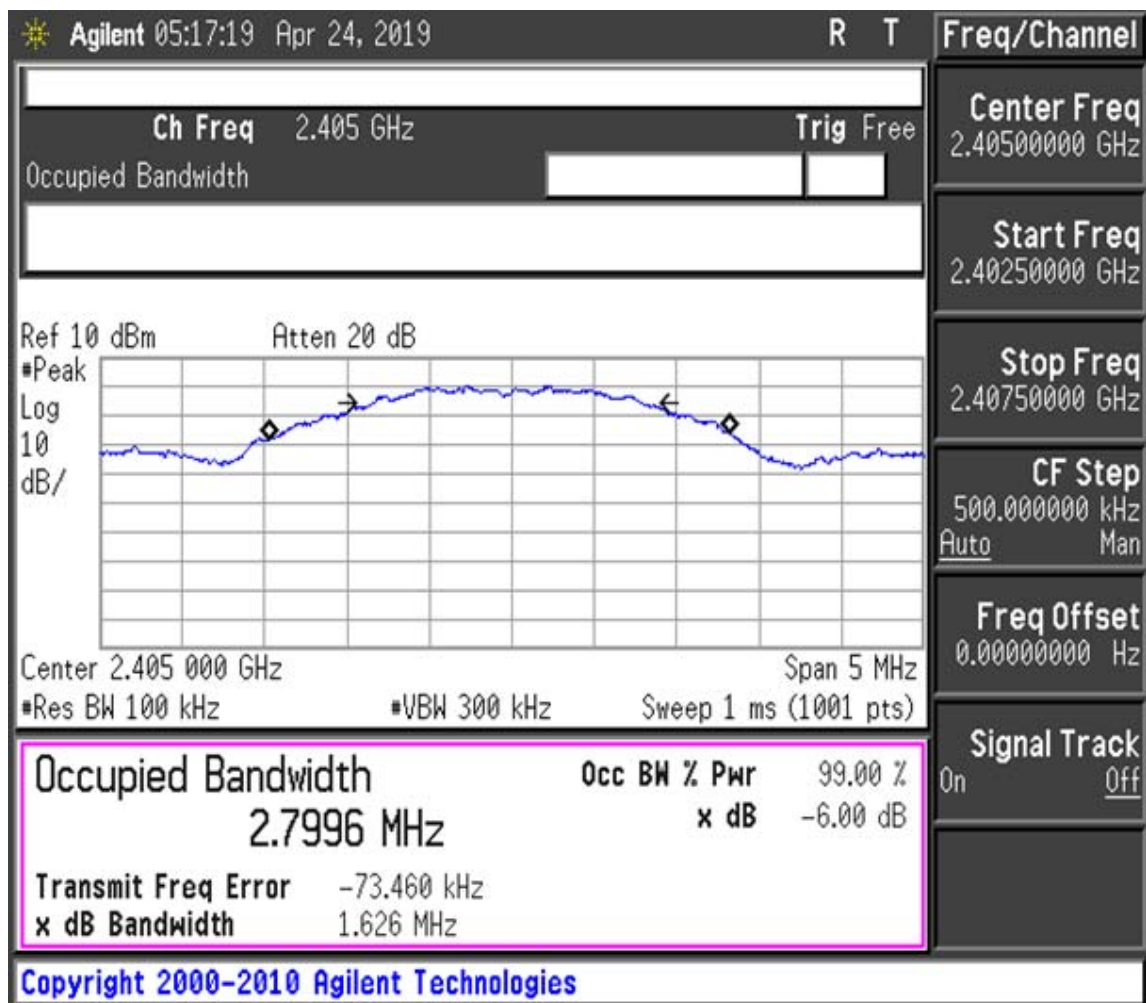
Figure 1. Plot of the 6dB Bandwidth & Occupied Bandwidth (99%)
