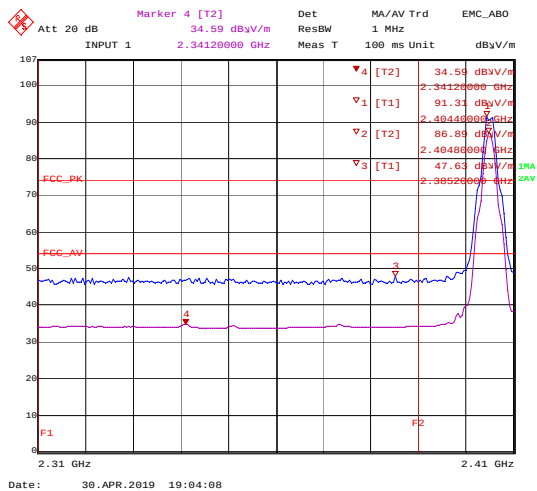
Figure 4. Plot of the Band Edge (Radiated)
