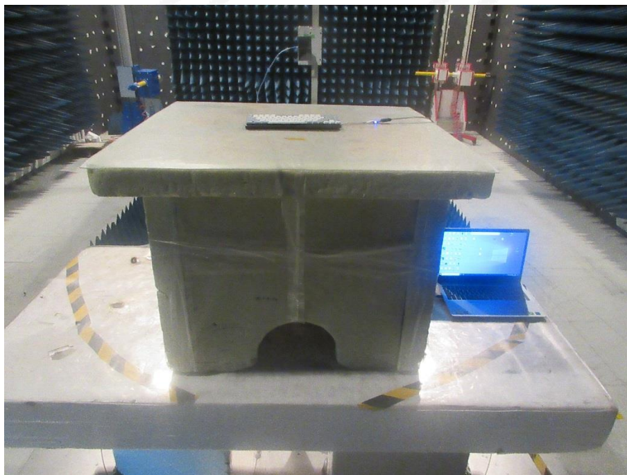
DXX&amp;DTS radiation H
