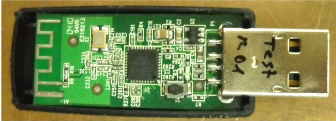
Photograph No.1 “RF dongle 2.4G” internal view
