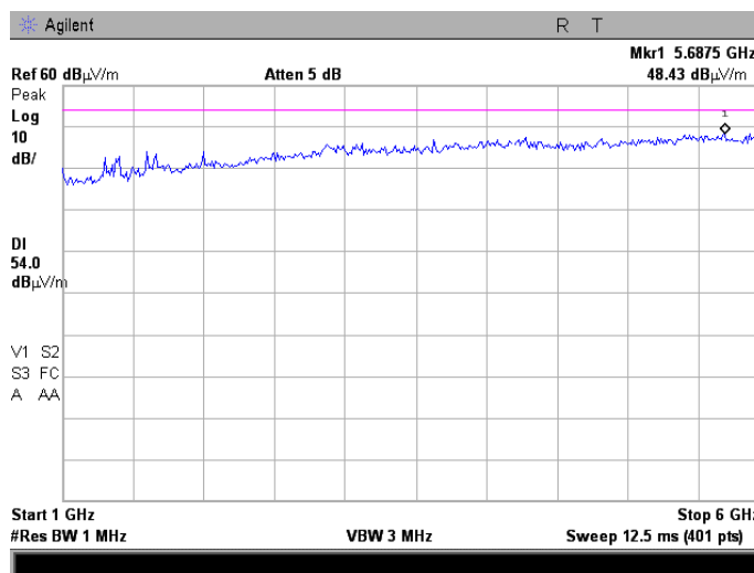
Plot 7.2.4 Radiated emission measurements in 1000 – 6000 MHz range, vertical antenna polarization
