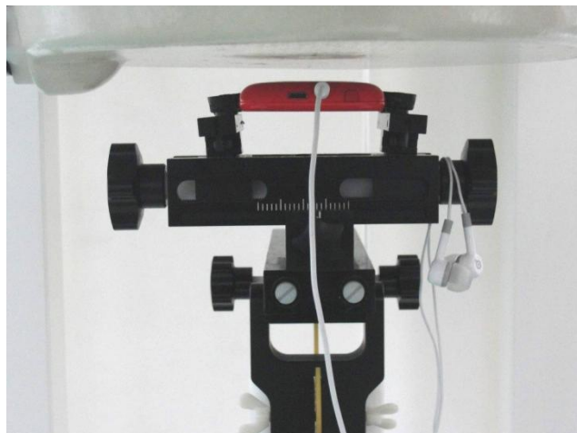
Rear Face of the DUT with Phantom 1 cm Gap (EUT with Earphone)
