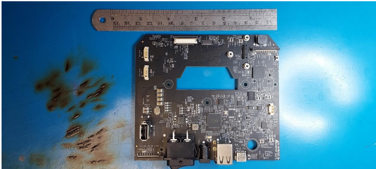
main board top view
