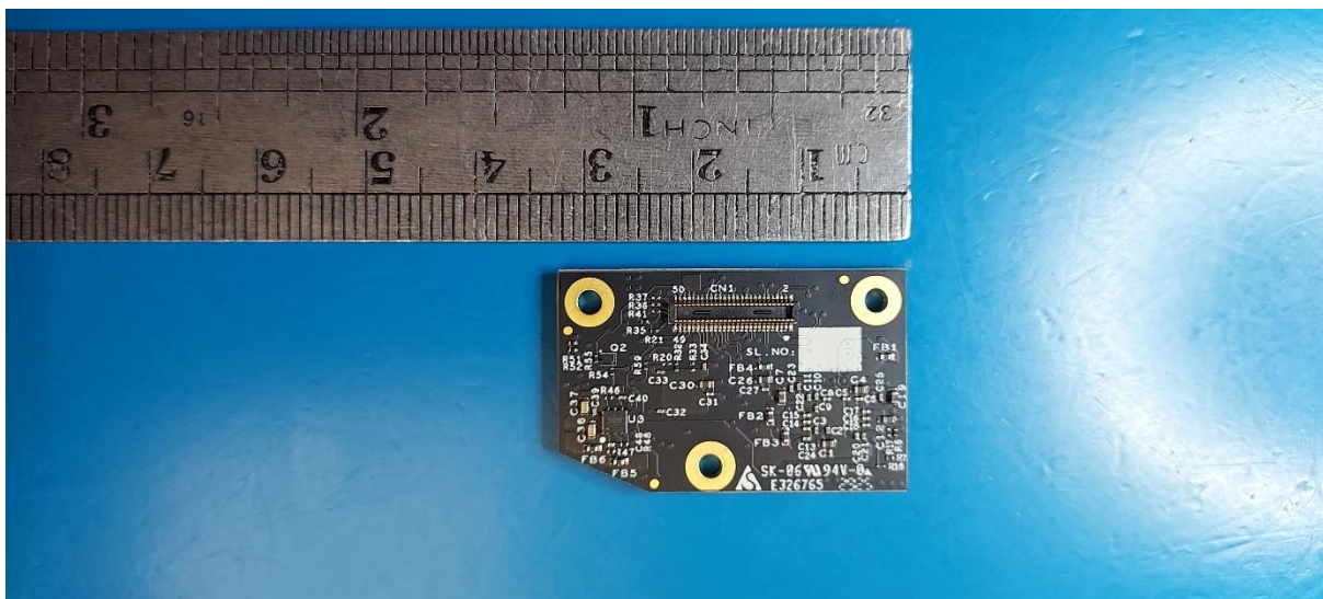
ISP Module board underside view
