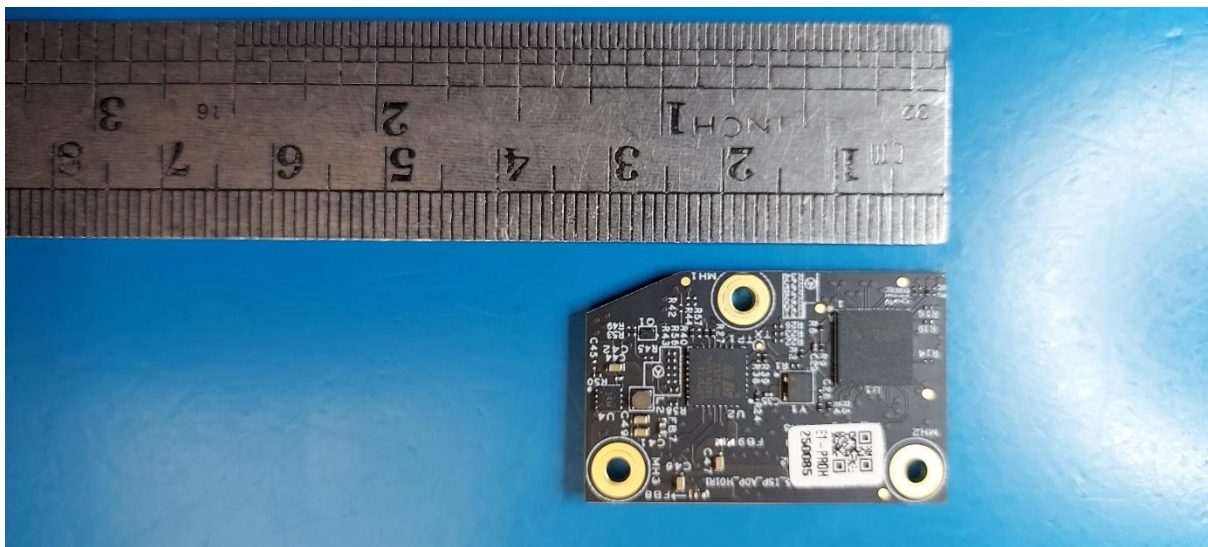
ISP Module board top view
