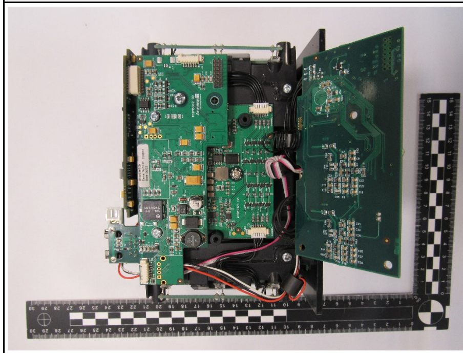
PCB Internal.view
