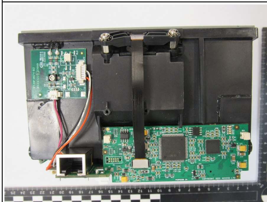
EUT Internal back view
