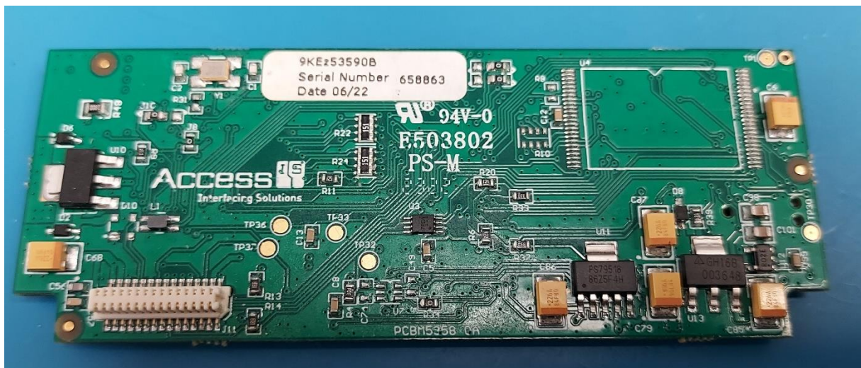
PCBM5358 ocr640 CAMERA rear
