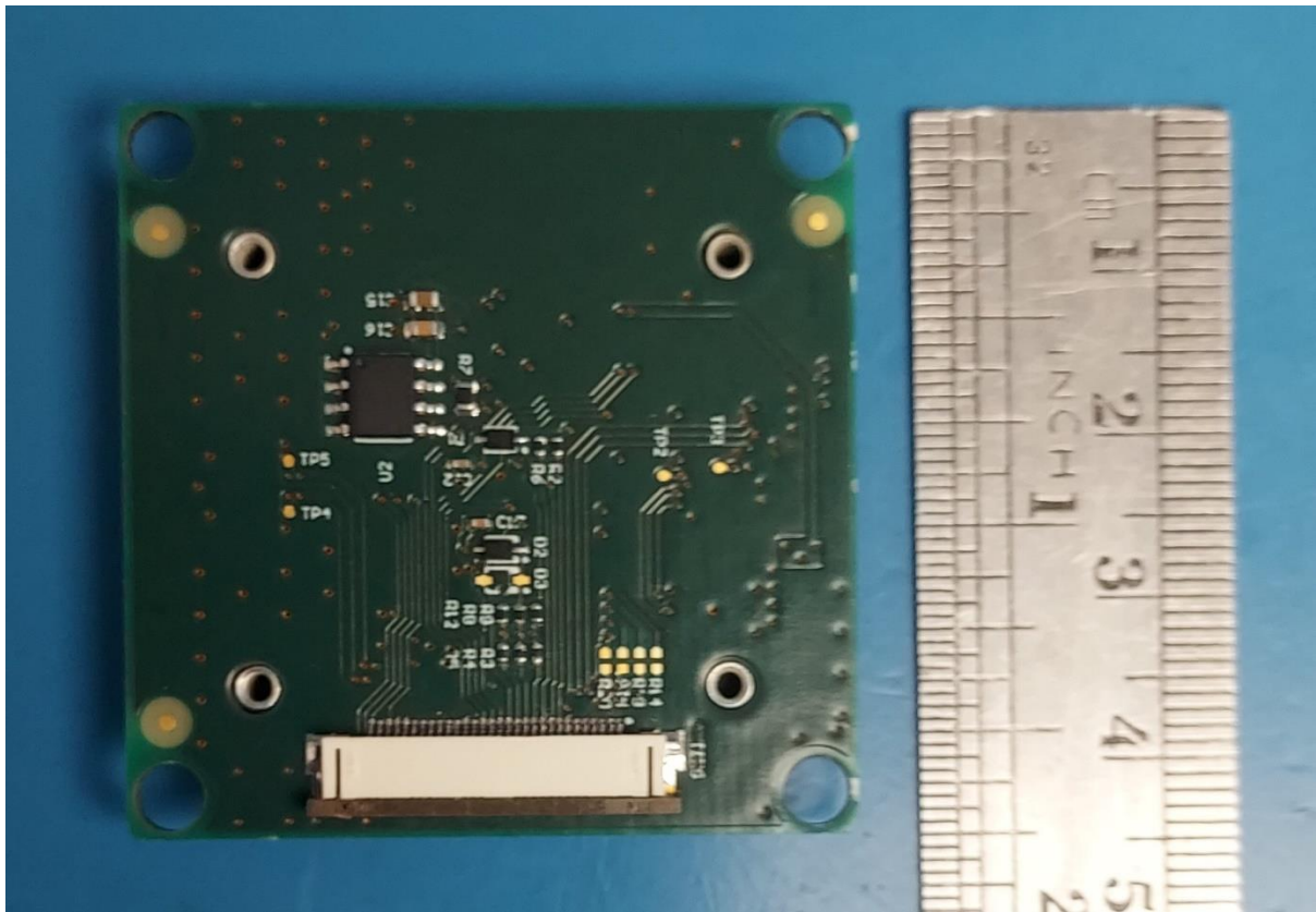
Reader adapter board Underside view
