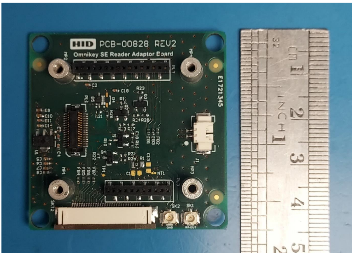
Reader adapter board Top view
