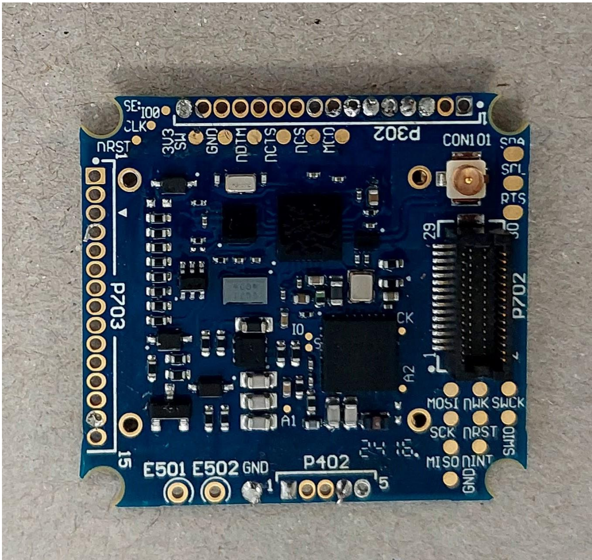
RFID module shielding removed view
