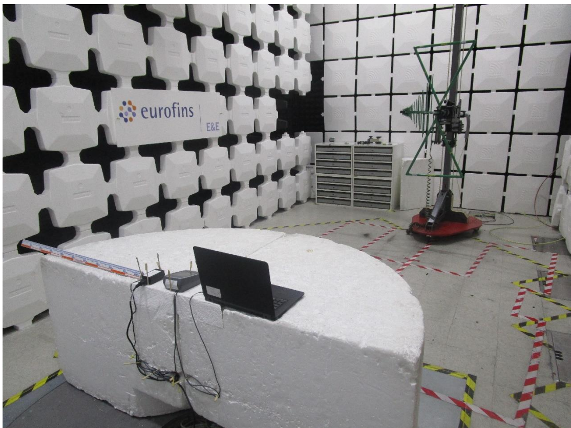
Radiated emissions 30MHz to 1GHz
