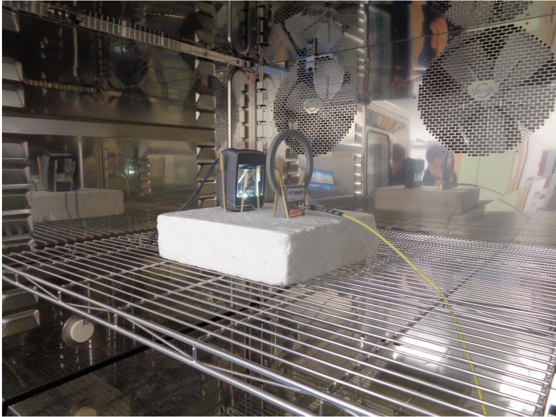
Arrangements for frequency tolerance tests – Test fixture – Environmental oven
