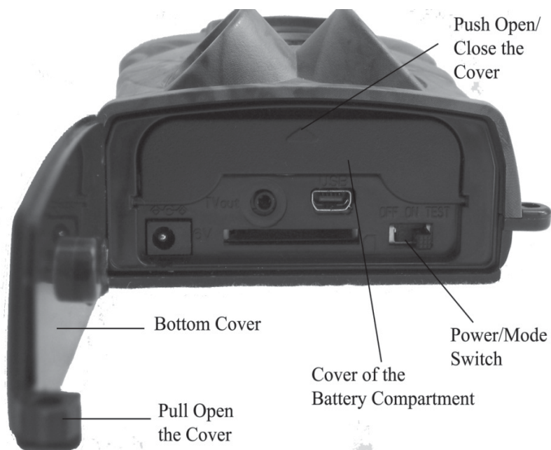
Figure 1.2: Bottom View of Ltl-5310M
