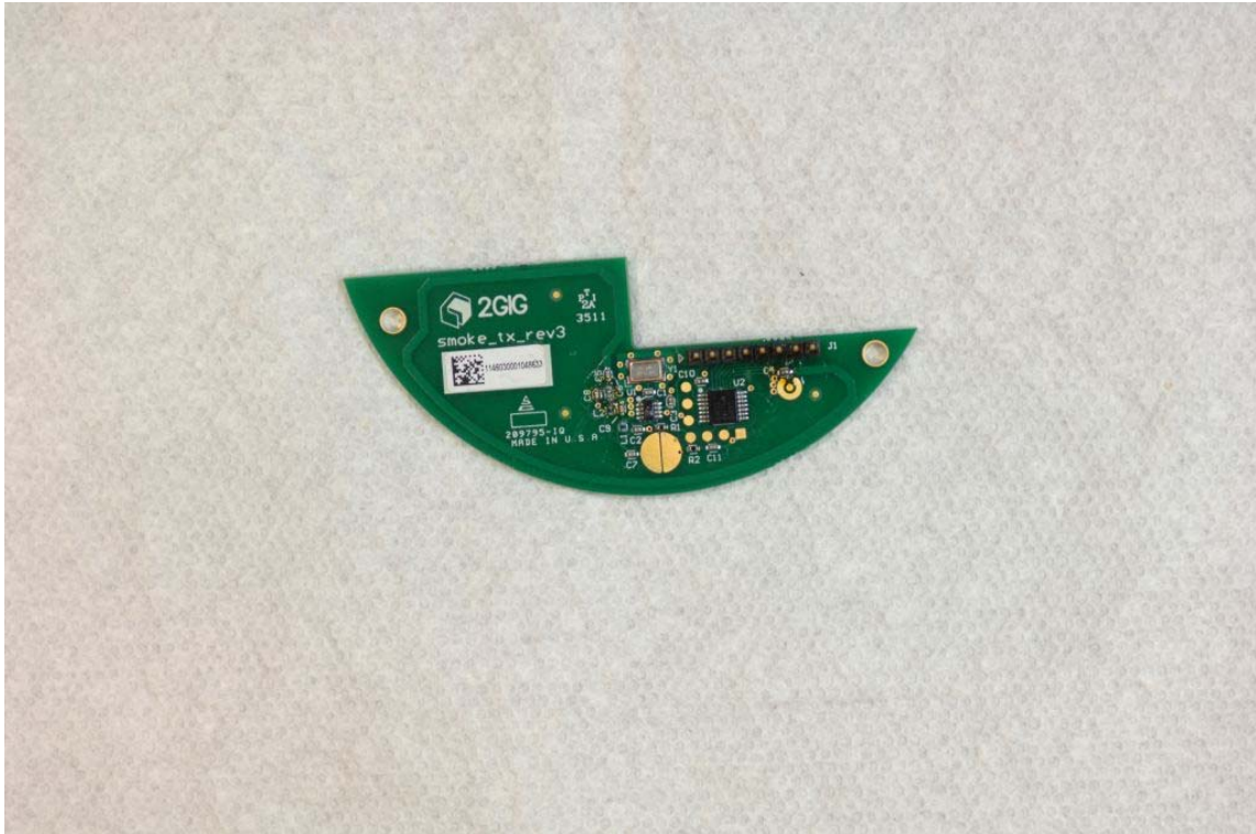
View of the Component Side of the Transmitter PCB
