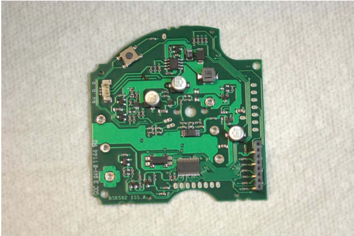
View of the Component Side of the Main PCB
