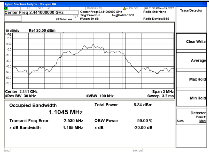
Channel 39 / 2441 MHz
