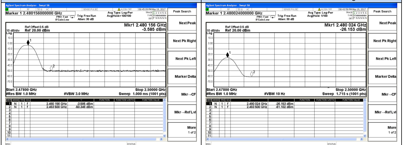
Channel 39 / 2480 MHz – Peak
