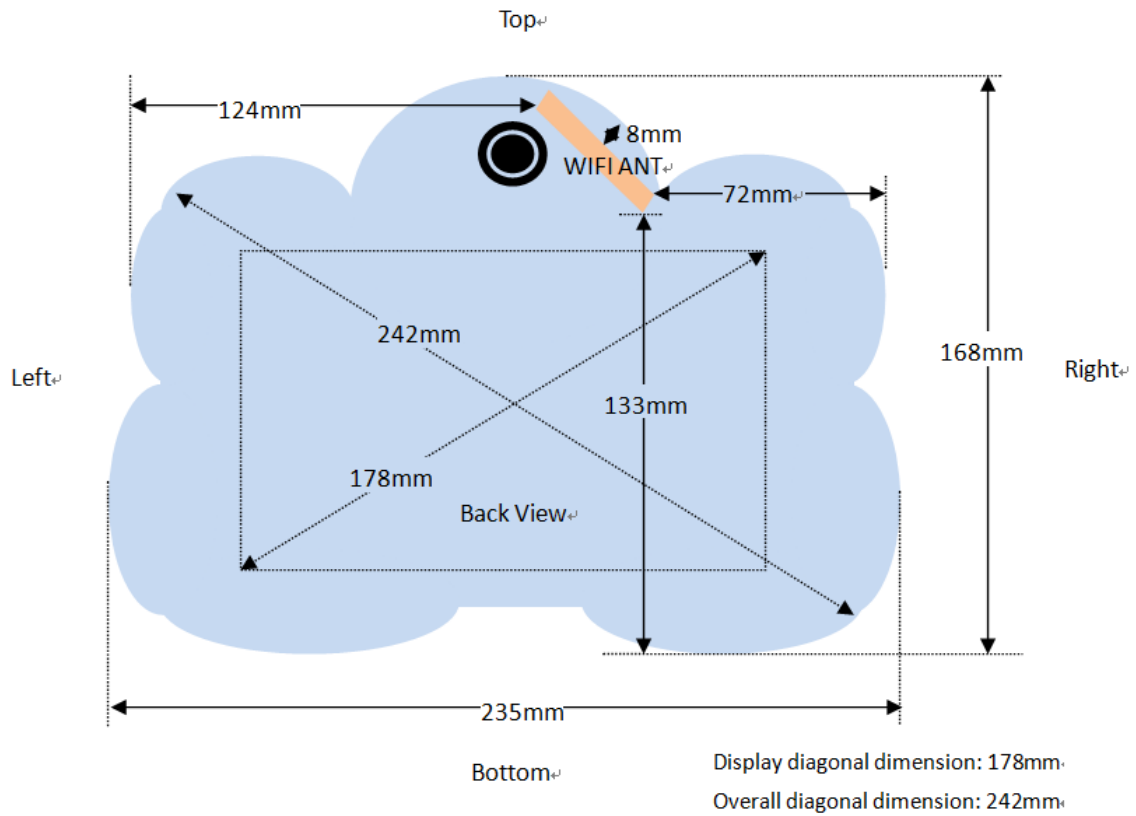
Fig.14.1 EUT Antenna Locations
