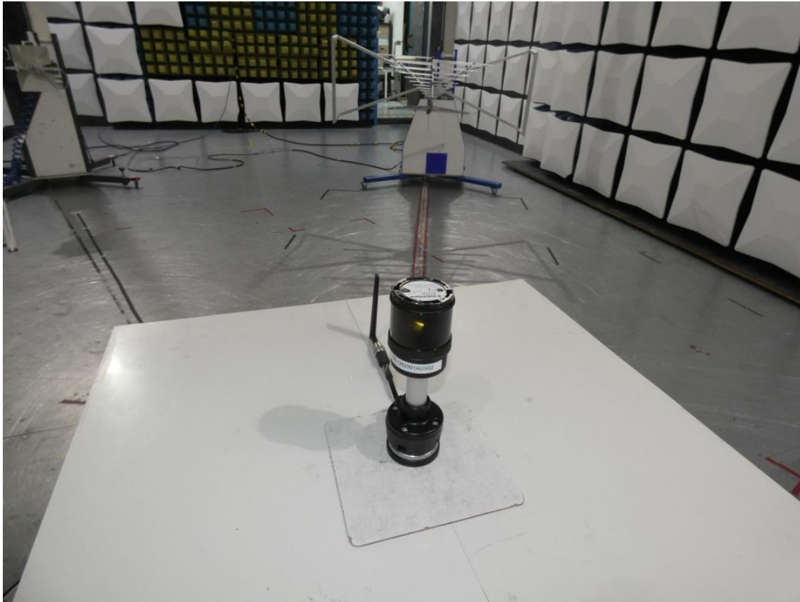
Photo 3: Setup for radiated emissions < 1 GHz, general view
