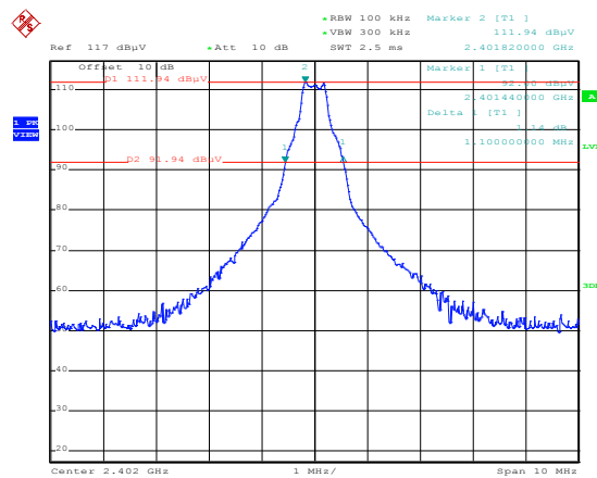
20dB Bandwidth CH00, 2402MHz
