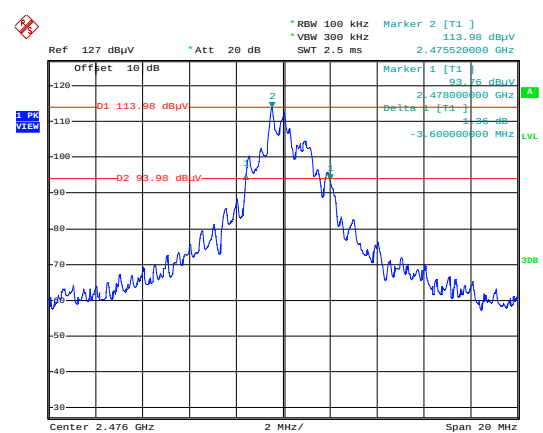
CH16, 2476MHz
