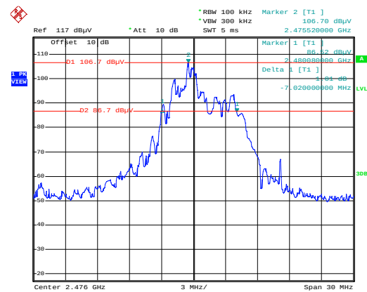
CH16, 2476MHz
