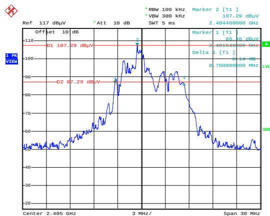
20dB Bandwidth CH01, 2405MHz
