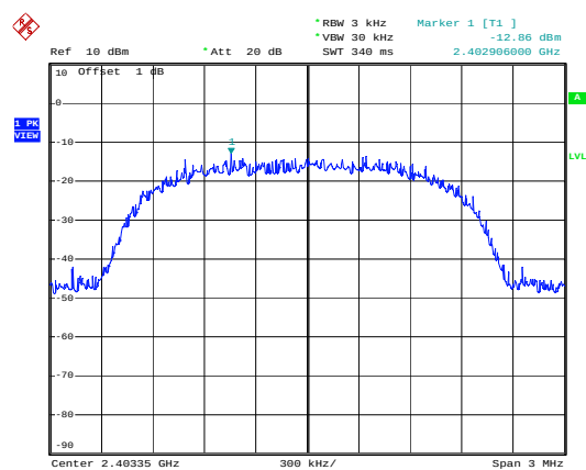
Modulation Type: GFSK, ANT 2 CH01
