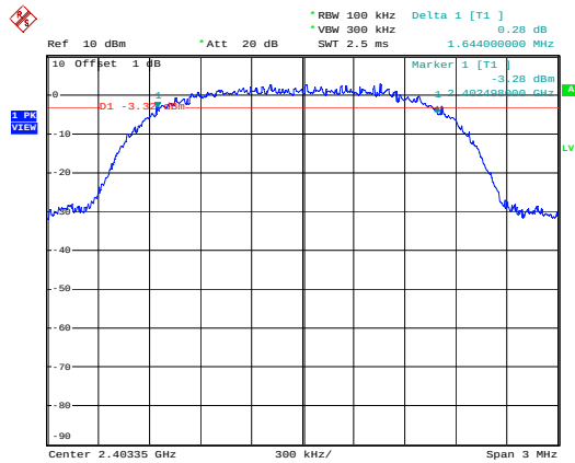
Modulation Type: GFSK, ANT 1 CH01
