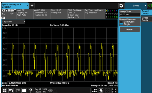
Period of Pulse Train
