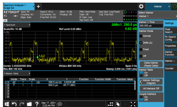
Pulse Time
