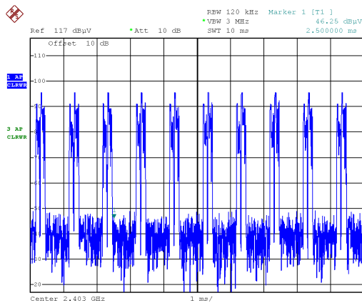
Period of Pulse Train
