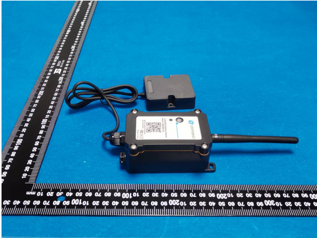
RS485-LB
